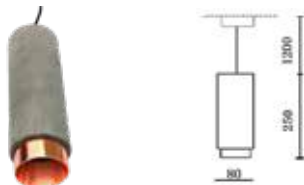
Fitting-Pendant Metal-1XGU10
