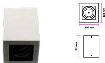
Fitting-Square-GU10
