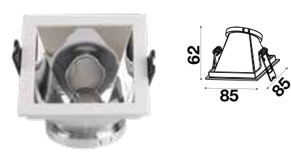
Fitting Square-GU10
