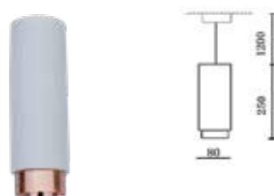
Fitting-Suspended-GU10
