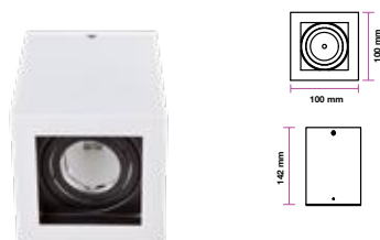
Fitting-Square-GU10
