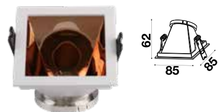
Fitting Square-GU10
