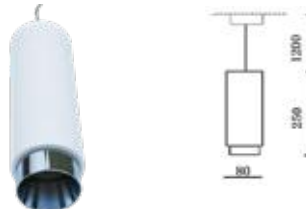
Fitting-Pendant Metal-1XGU10
