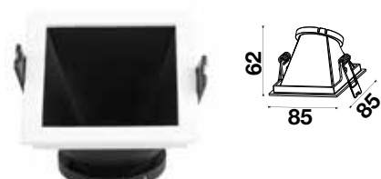
Fitting Square-GU10
