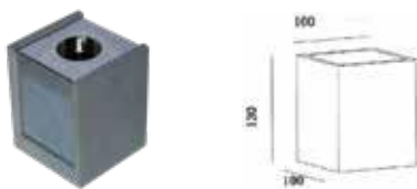
Fitting-Square Metal-1XGU10
