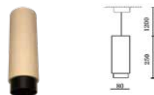
Fitting-Pendant Metal-1XGU10
