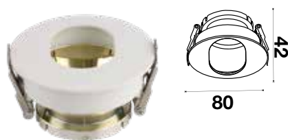
Fitting Round-GU10
